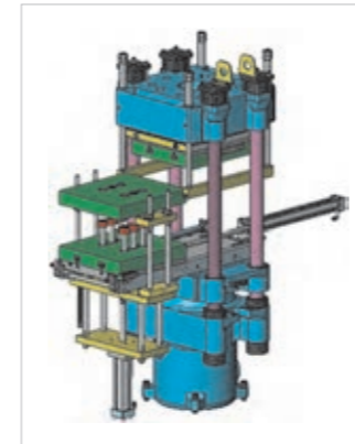
移模单层顶出 Sliding & Single-layer Ejecting
